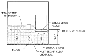
TYP. LAV. ELEVATION
