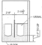
URINAL ELEVATION
