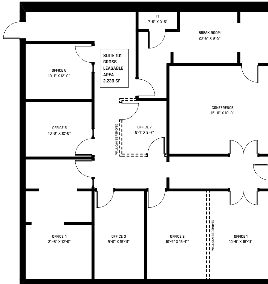
1 SUITE 101 SCALE: 3/32" = 1'-0"
