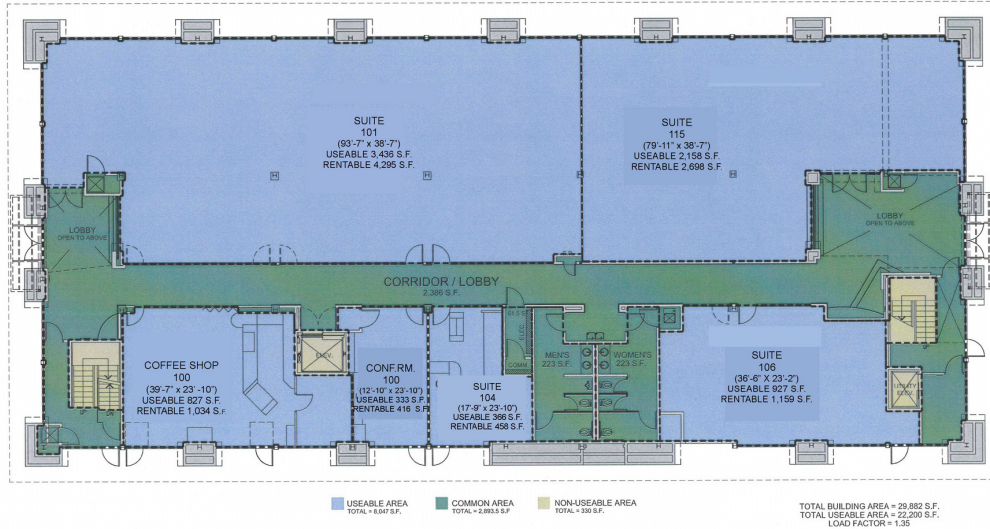
First Floor Plan - The 500 Building
