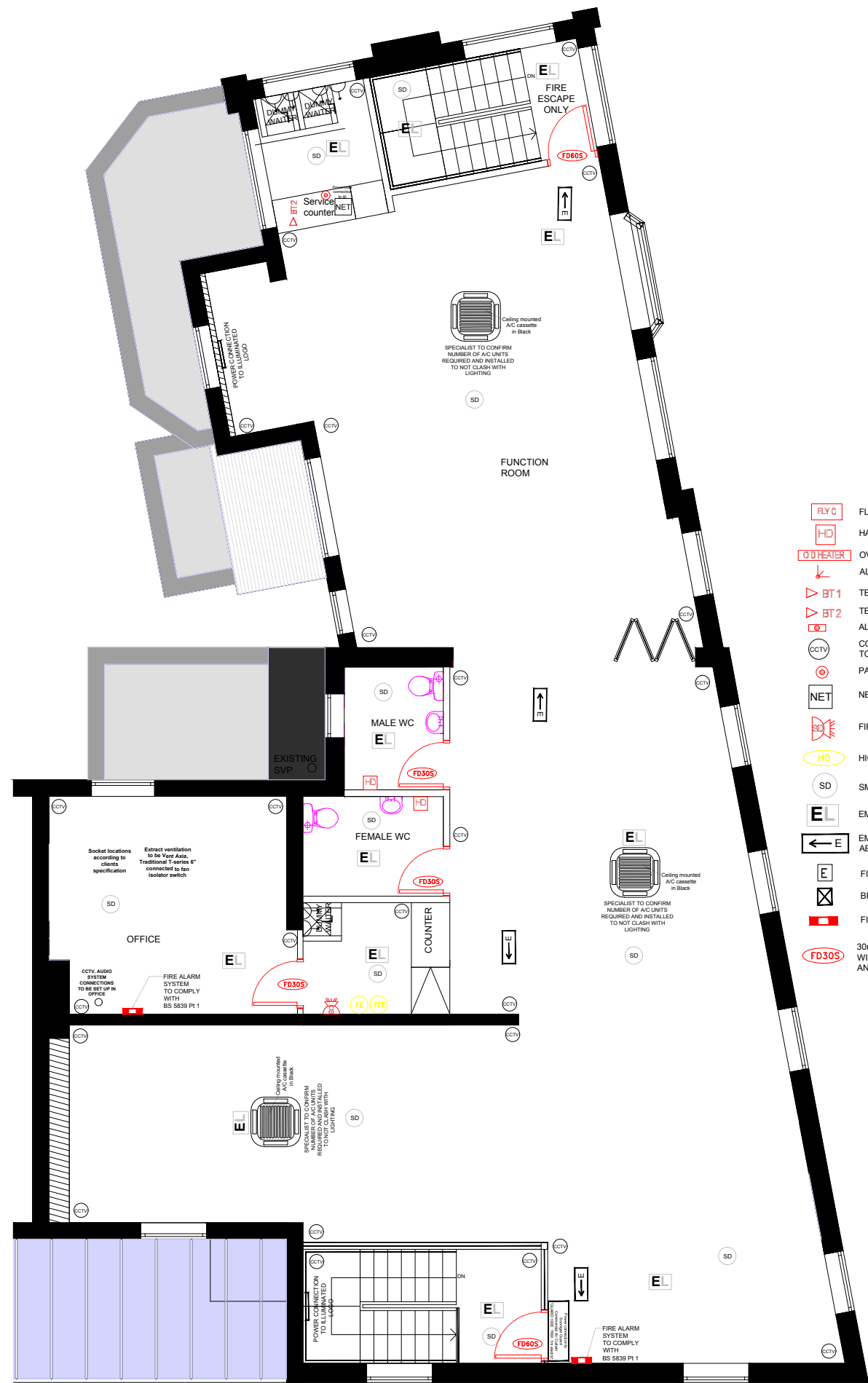
PROPOSED FIRST FLOOR ELECTRICAL LAYOUT
