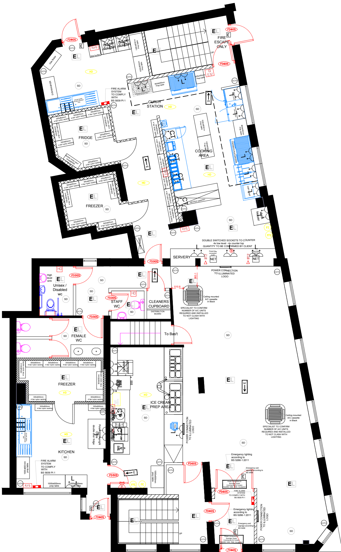
PROPOSED GROUND FLOOR ELECTRICAL LAYOUT
