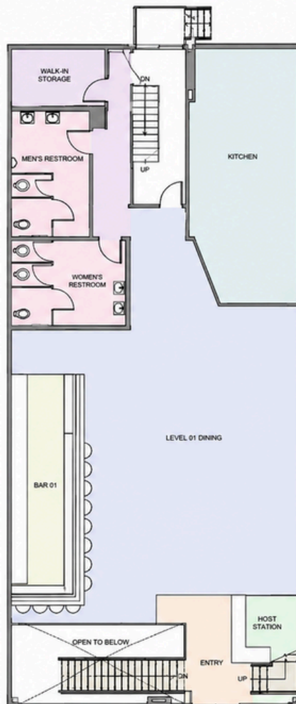
PLAN - LEVEL 01
