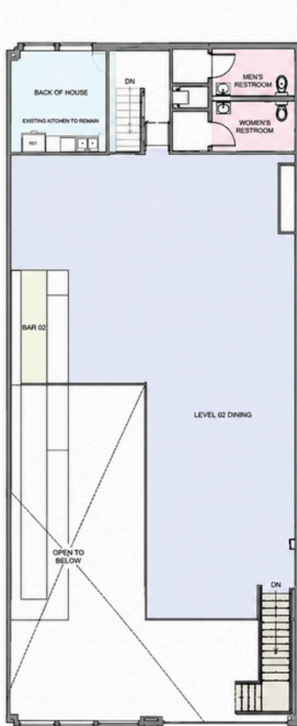
PLAN - LEVEL 02
