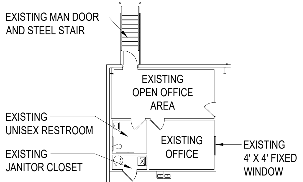
ENLARGED EXISTING OFFICE PLAN (APPROX. 510 S.F.)
