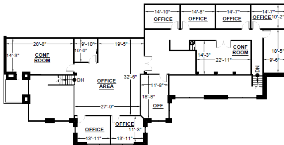
SECOND FLOOR
