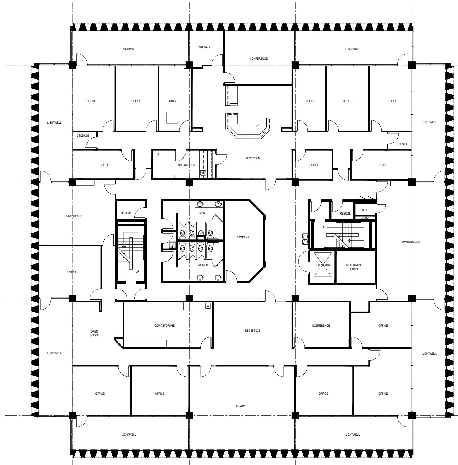
1 As-Built Floor Plan - Level 2
