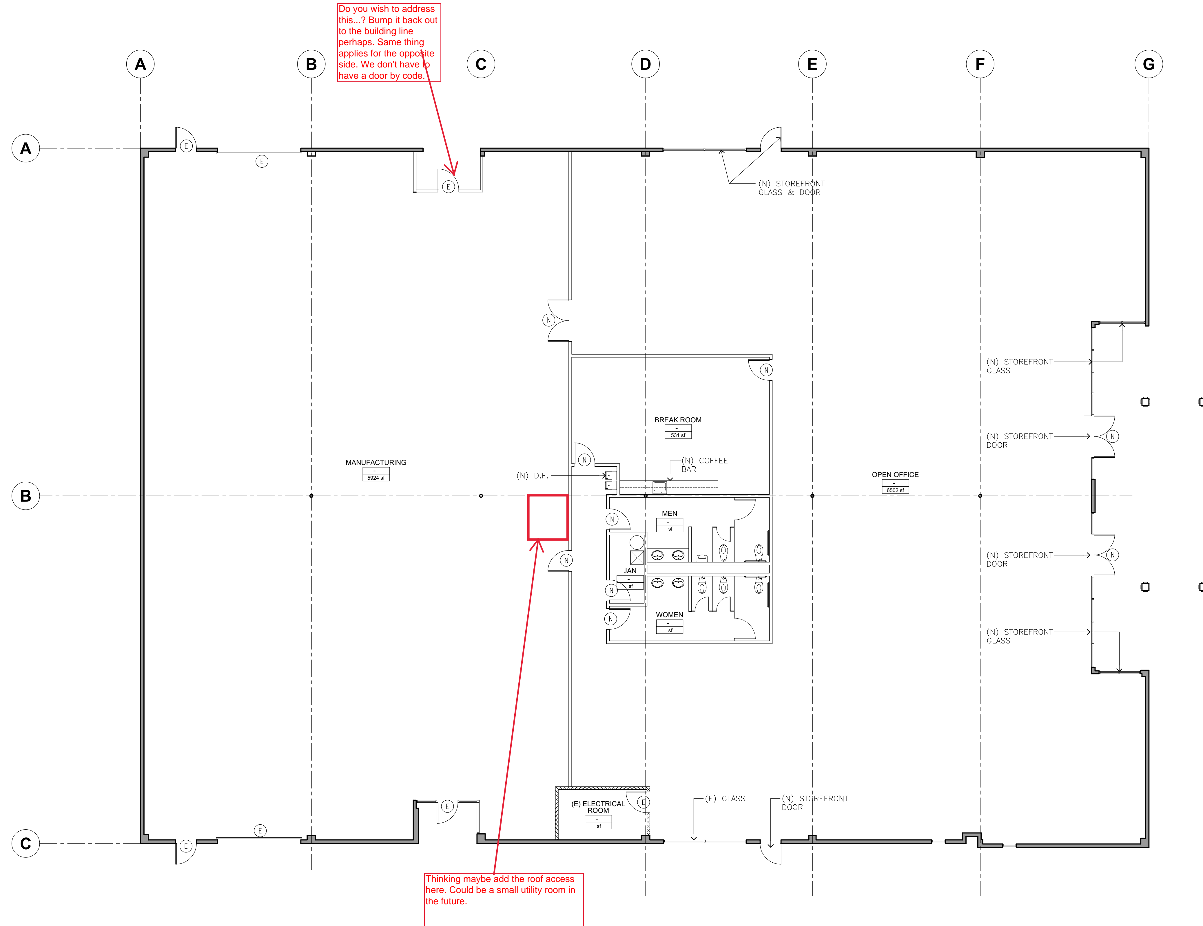
1 PRELIMINARY FLOOR PLAN SCALE: 1/8" = 1'-0"
