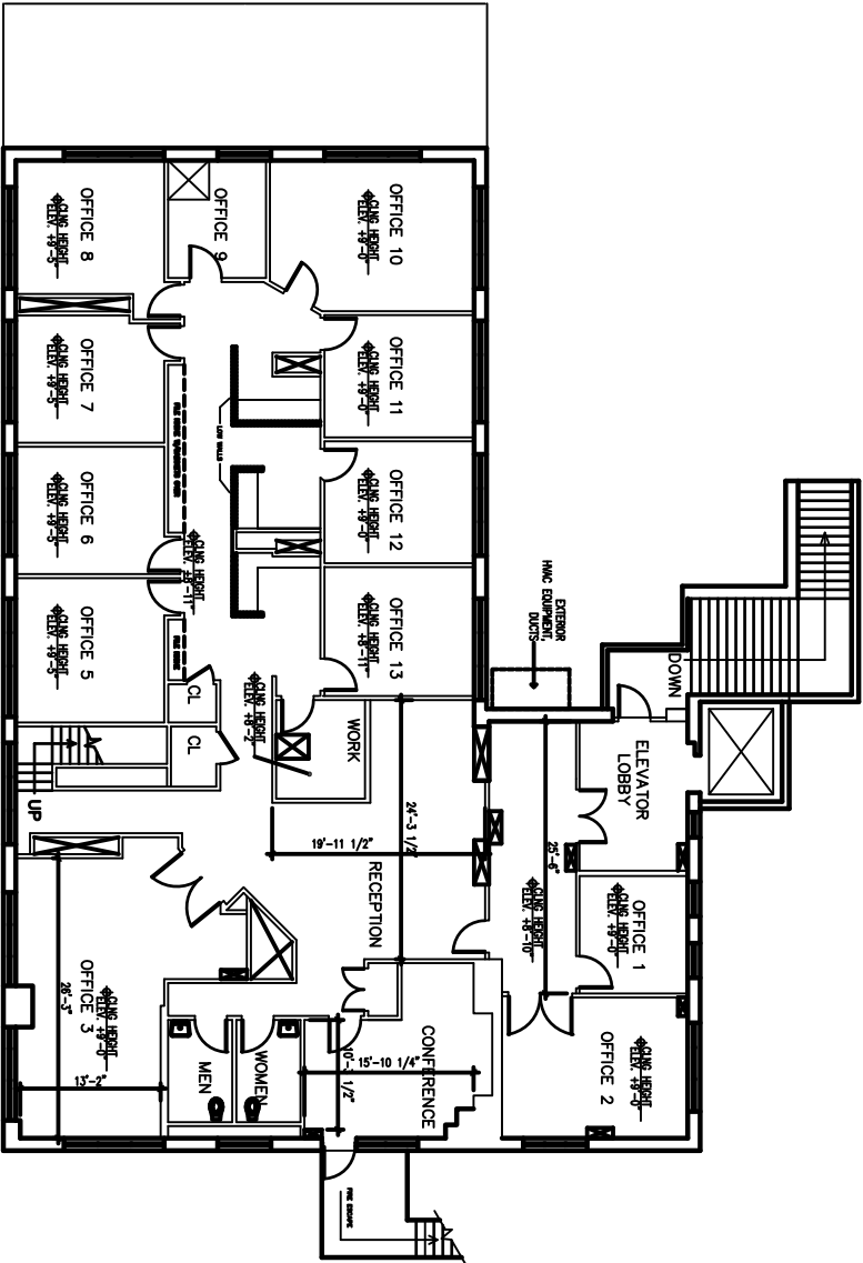
EXISTING 2ND LEVEL FLOOR PLAN ±15,000 SF
