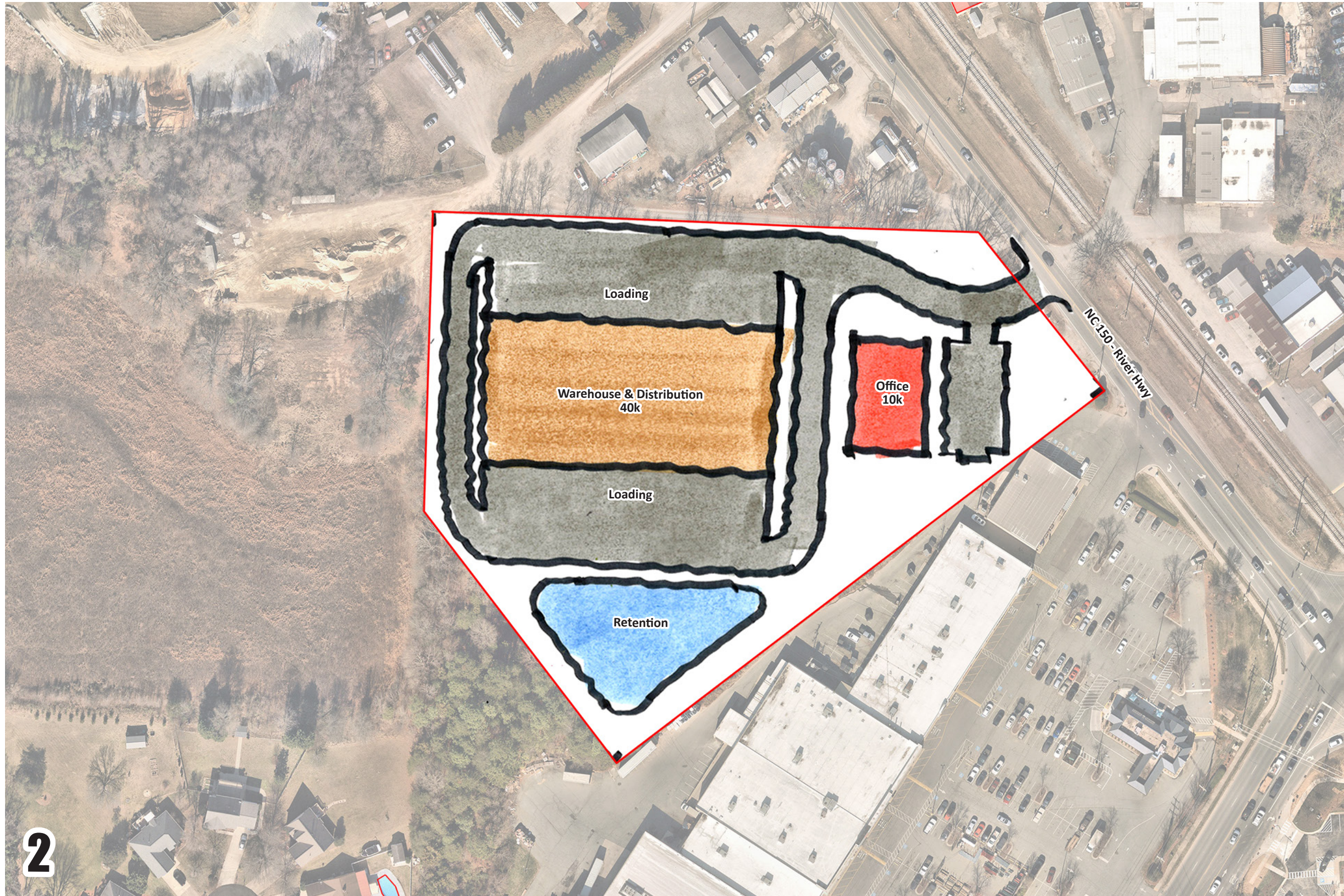
Light Industrial Layout
