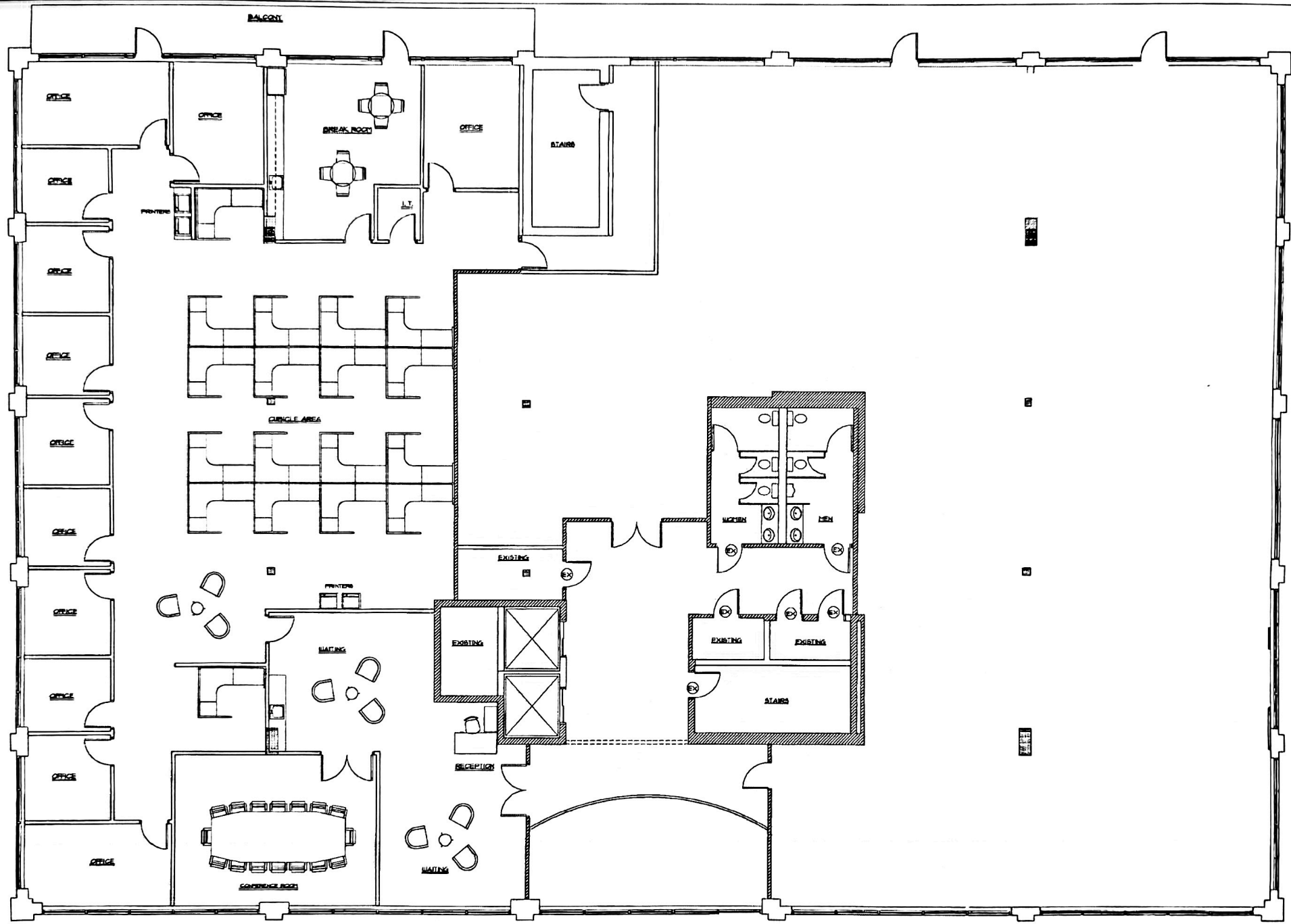
EXISTING FLOOR PLAN 5/16-11-07
