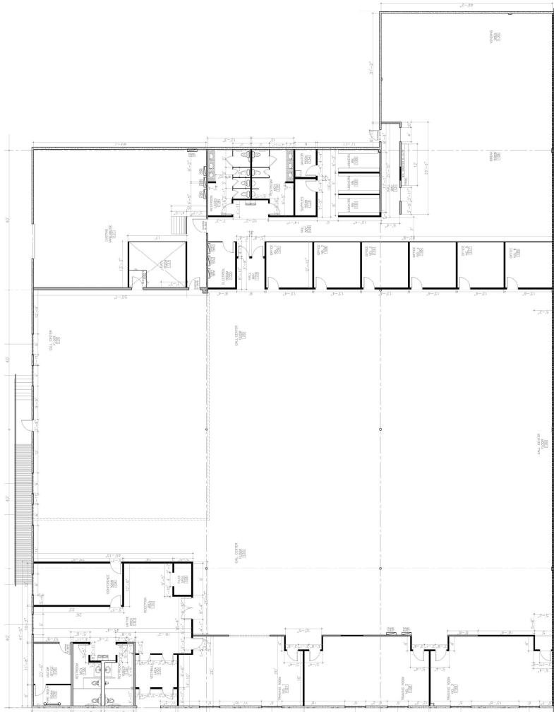
DEVELOPED FLOOR PLAN
