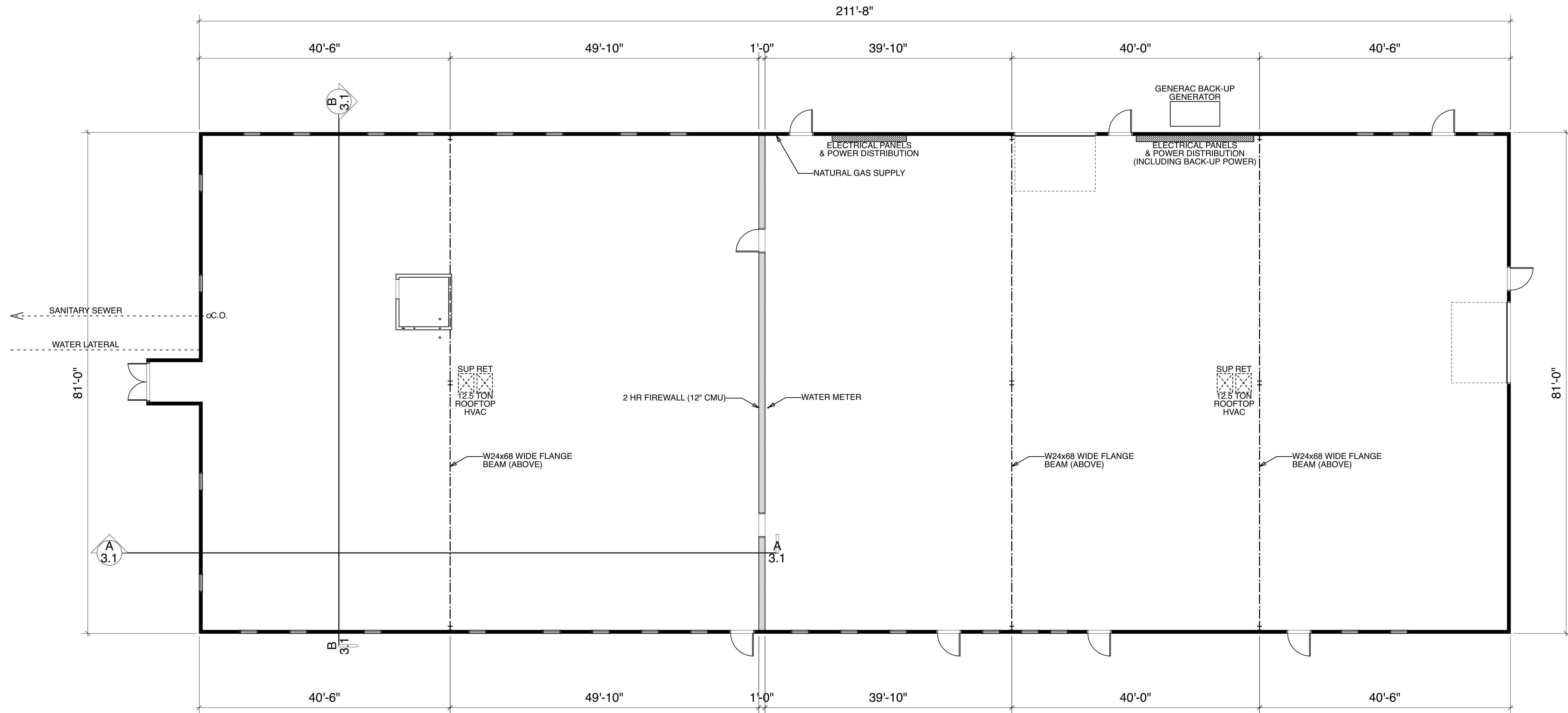
EXISTING FLOOR PLAN SCALE: 1/8" = 1'-0" 16,780 SQ. FT. (INTERIOR DIMENSIONS)
