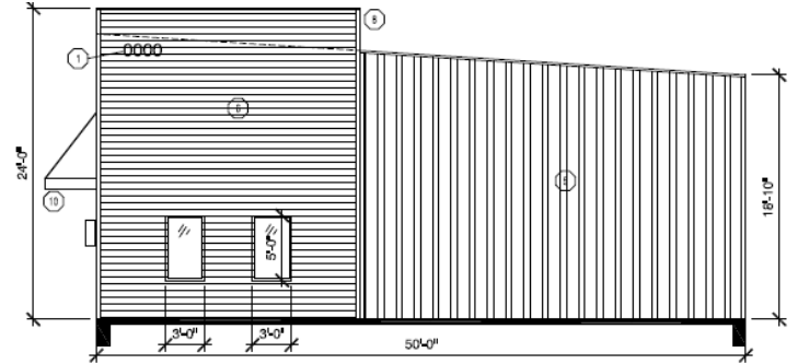
BLDG 1 - NORTH ELEVATION
