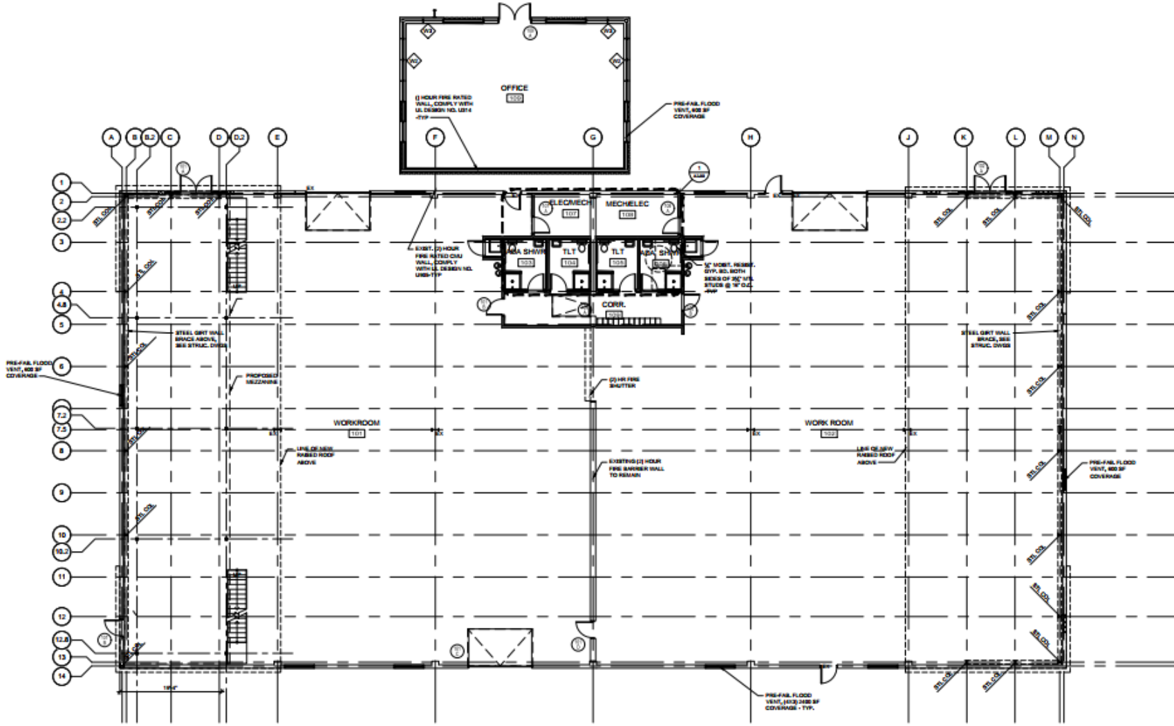
GROUND FLOOR PLAN SCALE: 1/4" = 1'-0"
