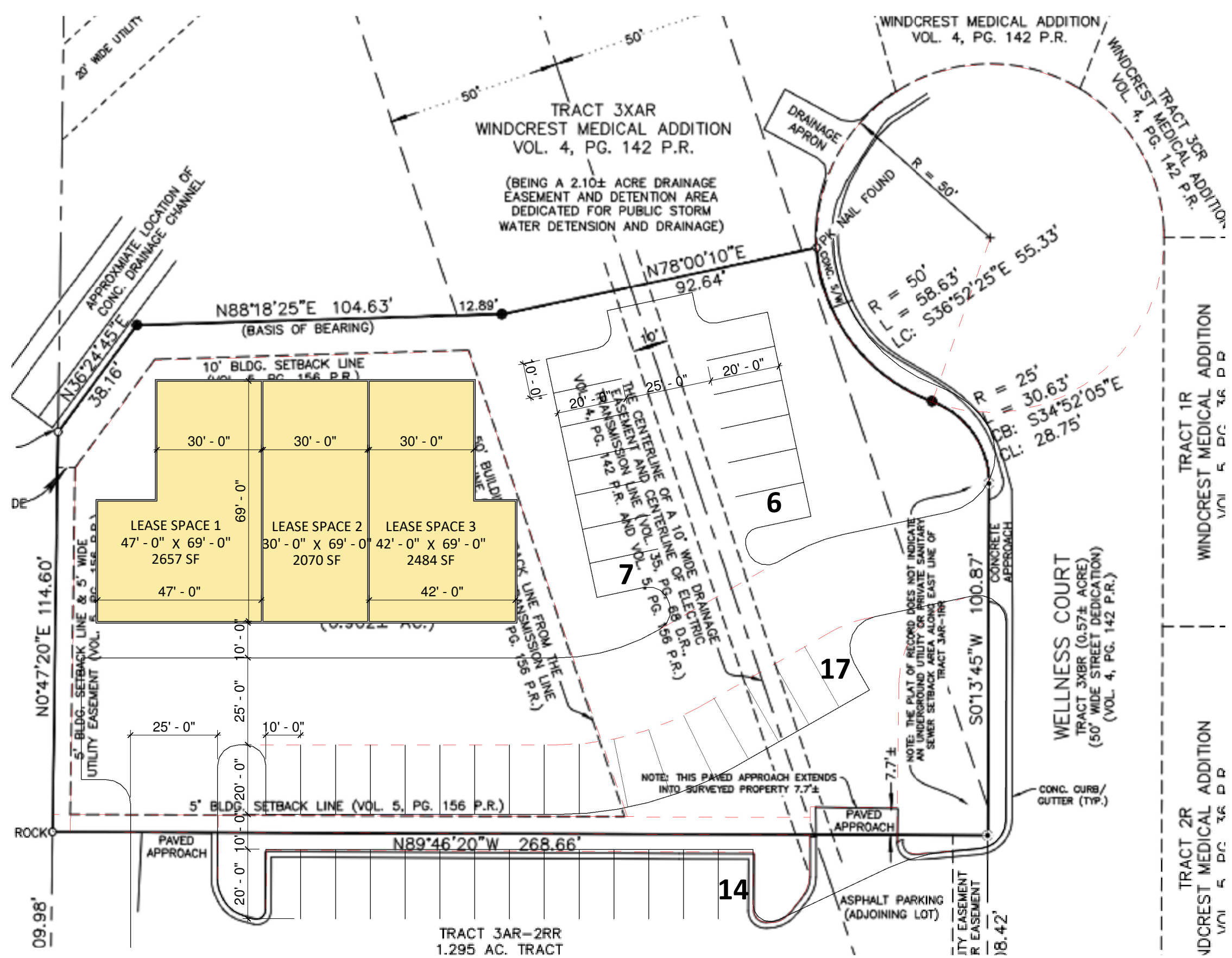
WELLNESS COURT SHELL BUILDING FLOOR PLAN - TEST FIT - OPT 2 1" = 30'-0"
