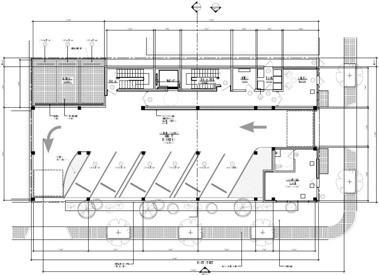
529-531 Mulberry Street Ground Floor Plan
