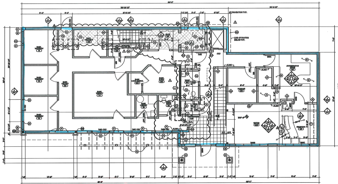
1 MAIN LEVEL FLOOR PLAN A2.1 1/4"=1'-0"
