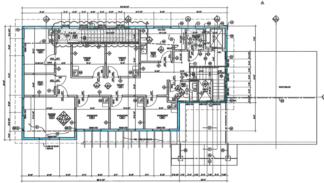
1 UPPER LEVEL FLOOR PLAN A2.3 1/4"=1'-0"
