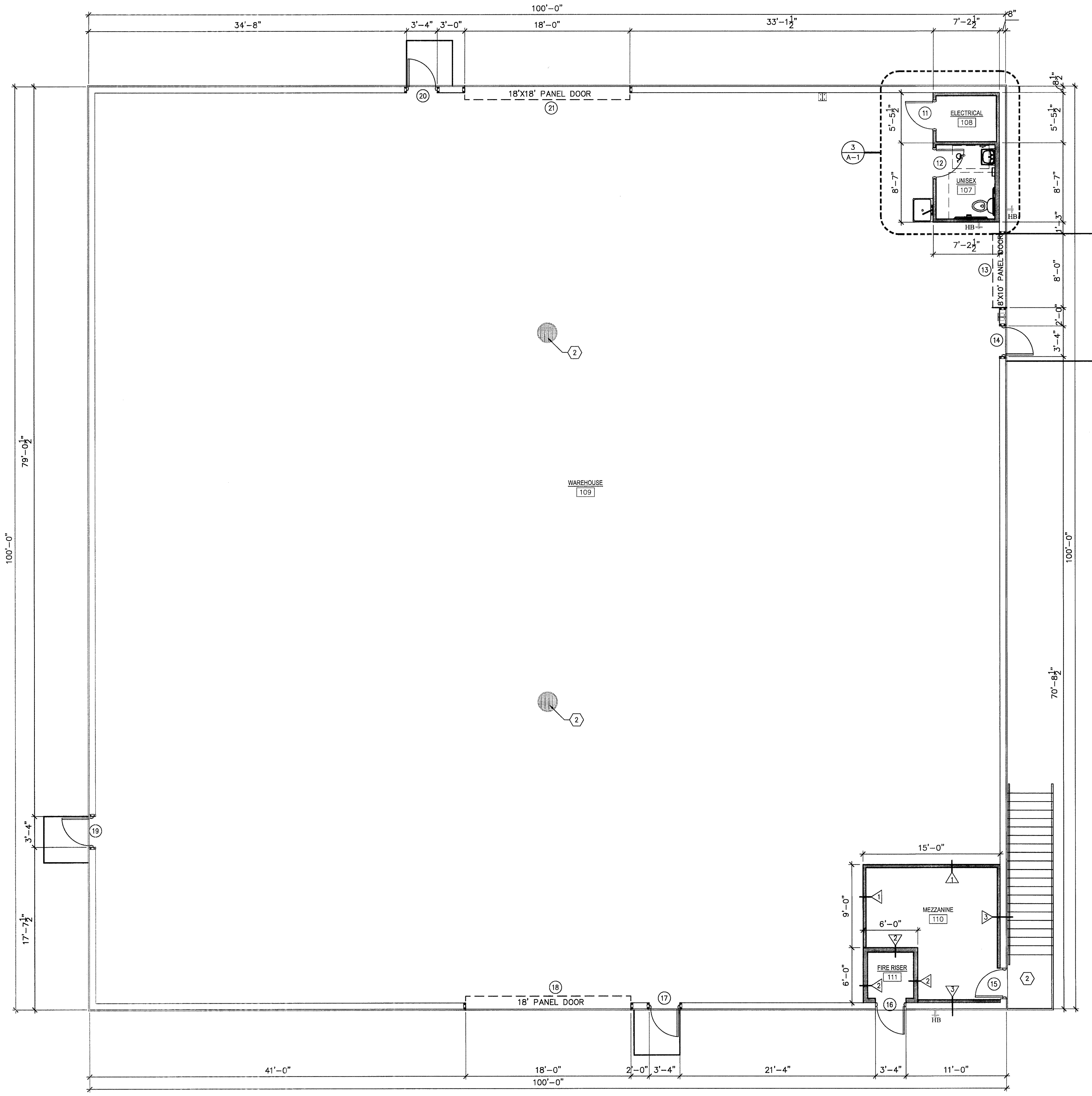
FLOOR PLAN "B" SCALE: 3/16" = 1'-0"
