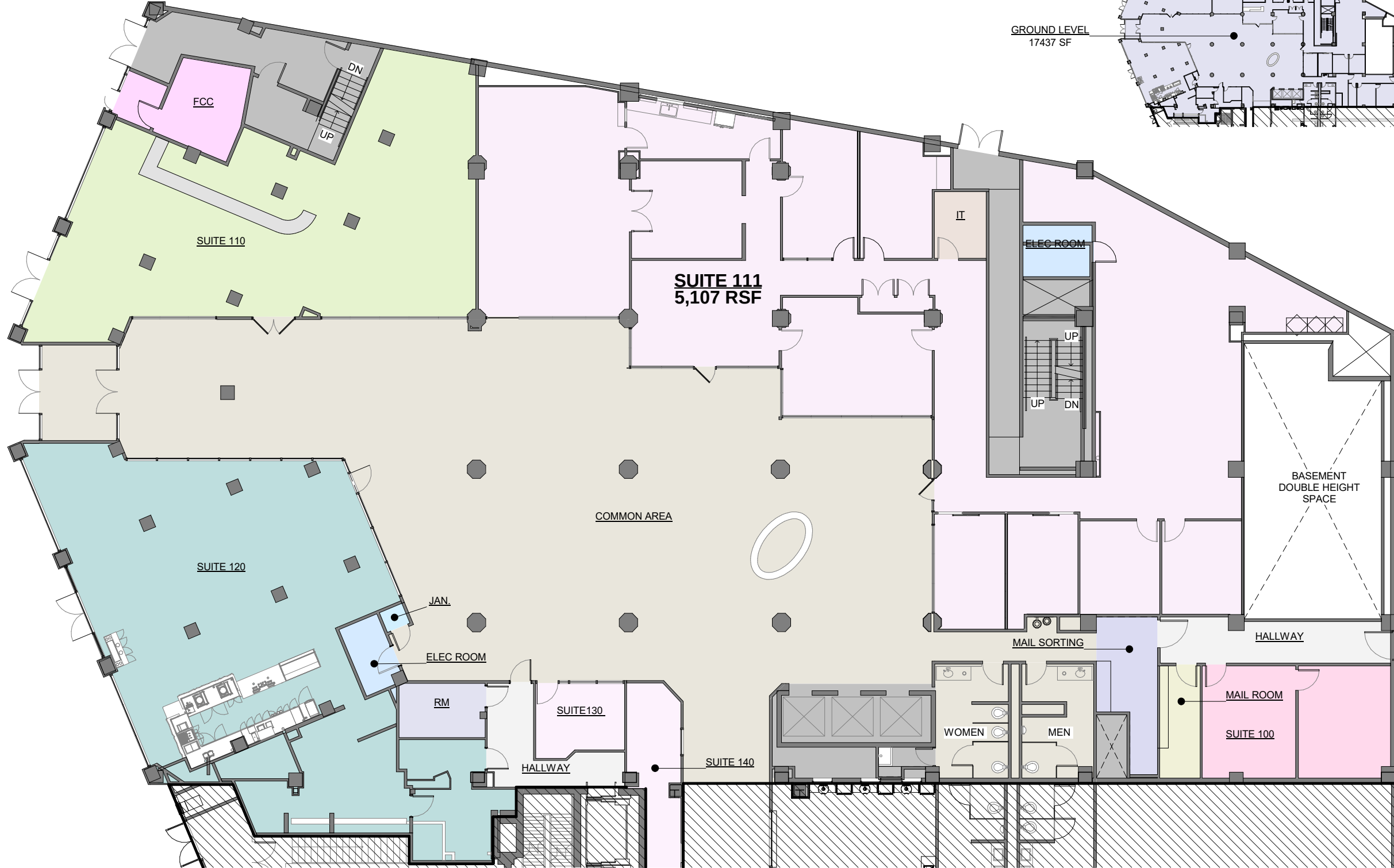
① CENTRE - GROUND FLOOR 1/16" = 1'-0"
