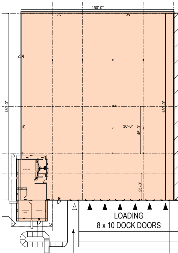
FLOOR PLAN - 28,866 SF
