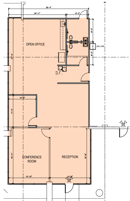
OFFICE PLAN - 1,760 SF
