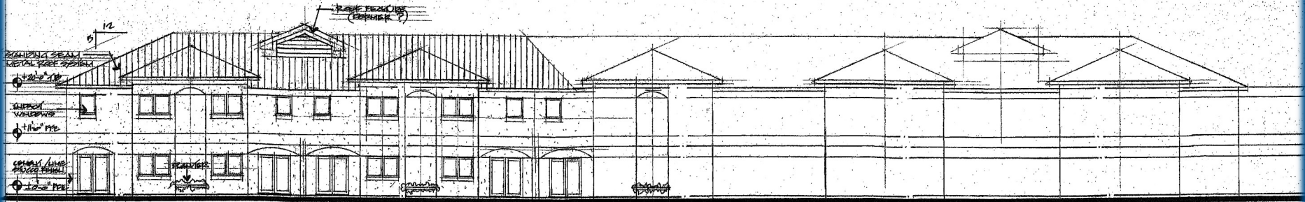
PARTIAL REAR ELEVATION (SPECIALTY BUILDING) (12-11-12)
