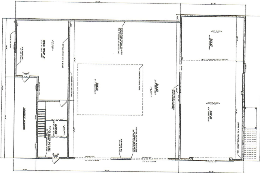
EXISTING GROUND LEVEL FLOOR PLAN
