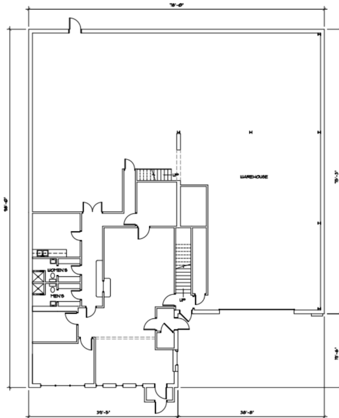
FIRST FLOOR PLAN SCALE: 1/8"=1'-0"
