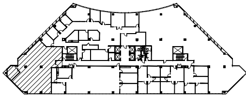
KEYPLAN - 5TH FLOOR
