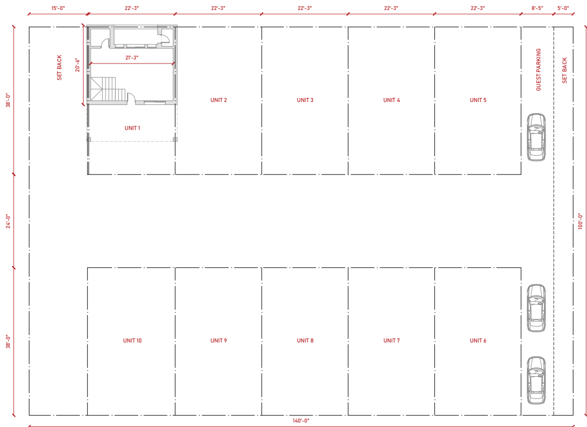
SITE PLAN SCALE: 1/16" = 1'-0"
