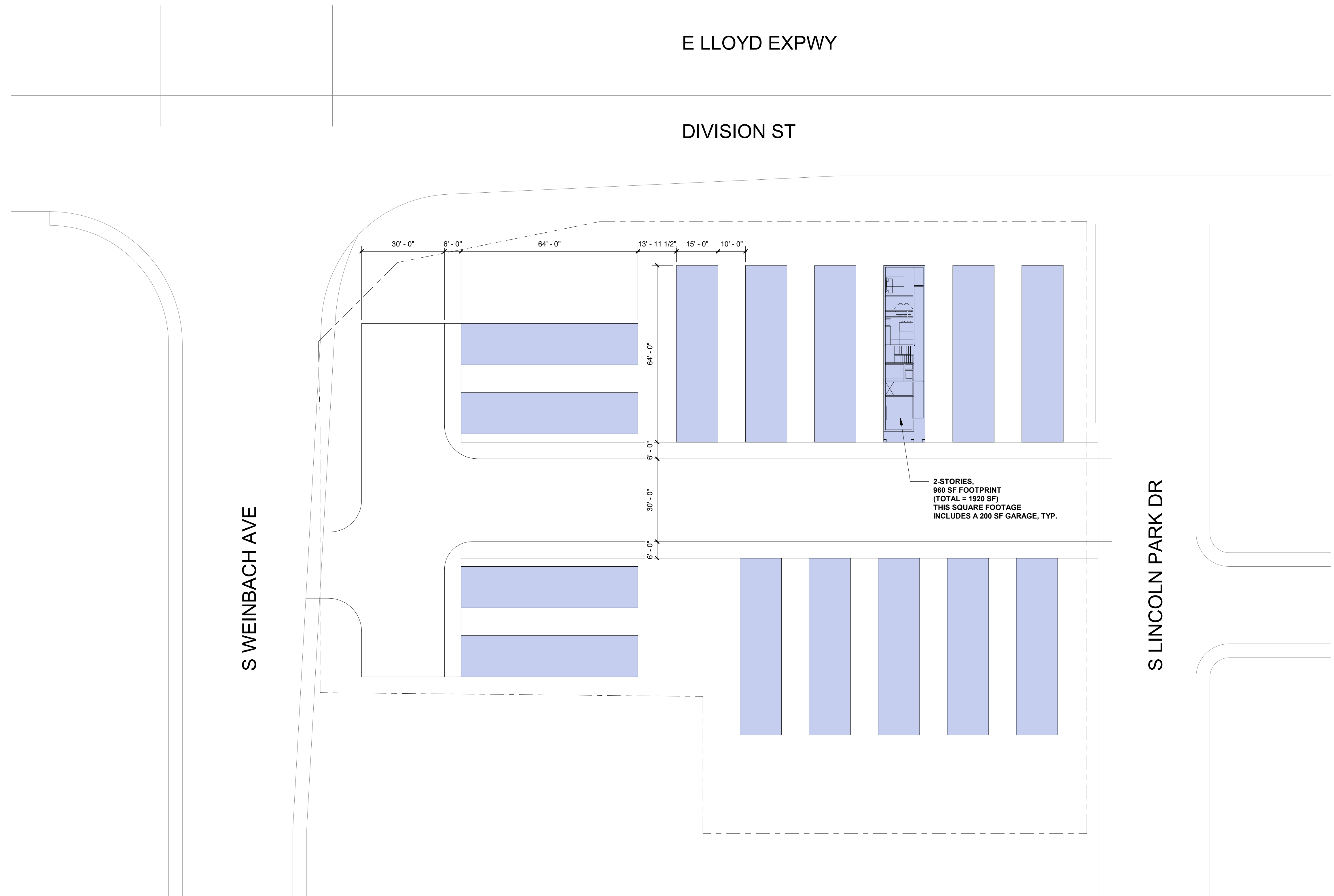
SITE PLAN 1" = 20'-0"
