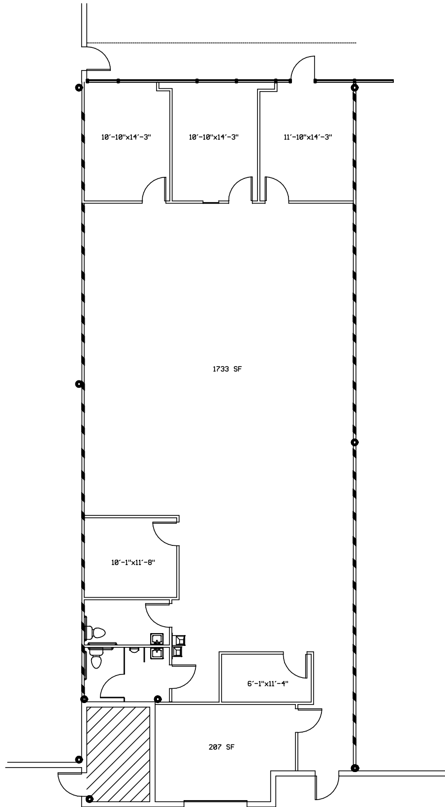
1 FLOOR PLAN COBB CORPORATE BLDG 375 SUITE 440
