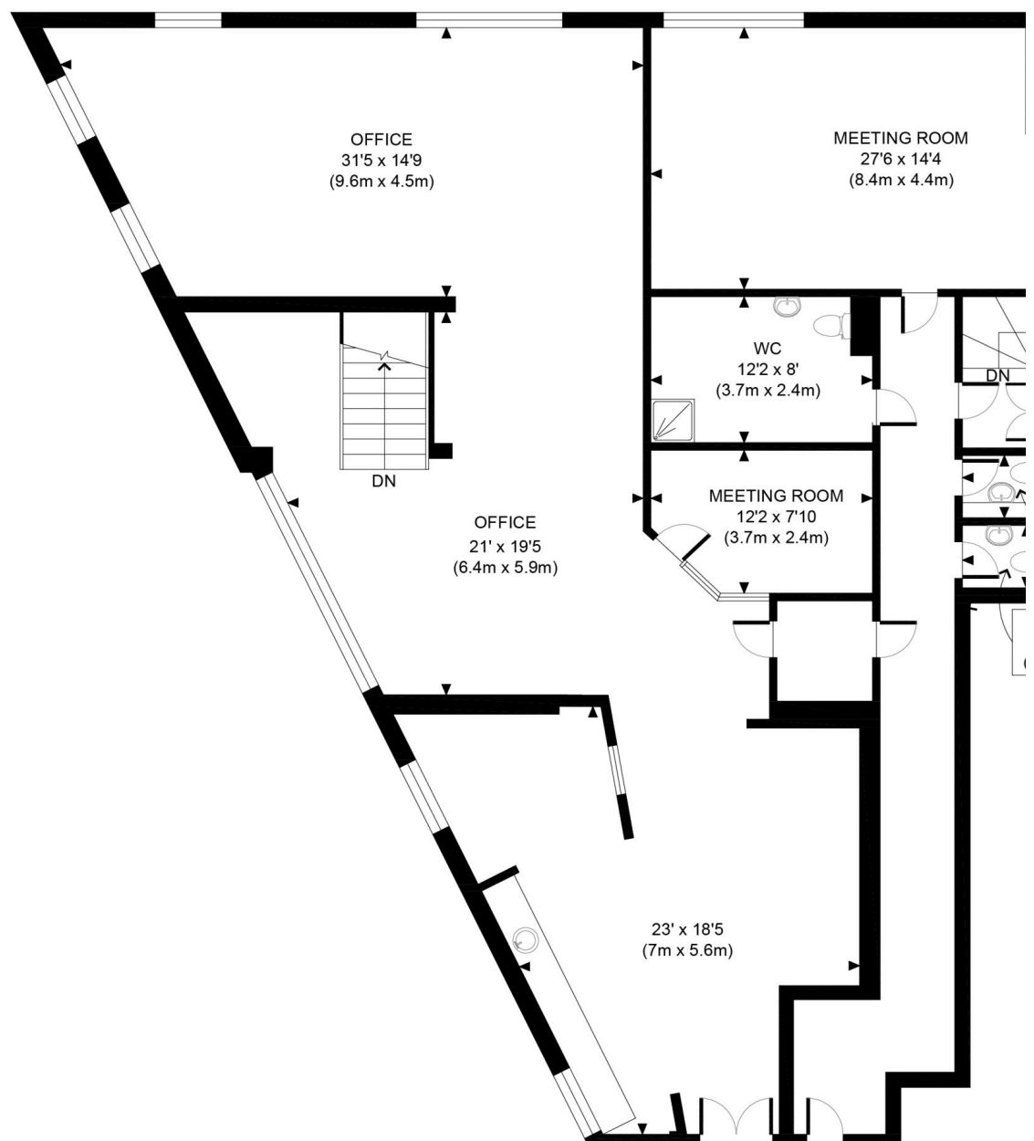
LOWER GROUND FLOOR GROSS INTERNAL FLOOR AREA 887 SQ FT
