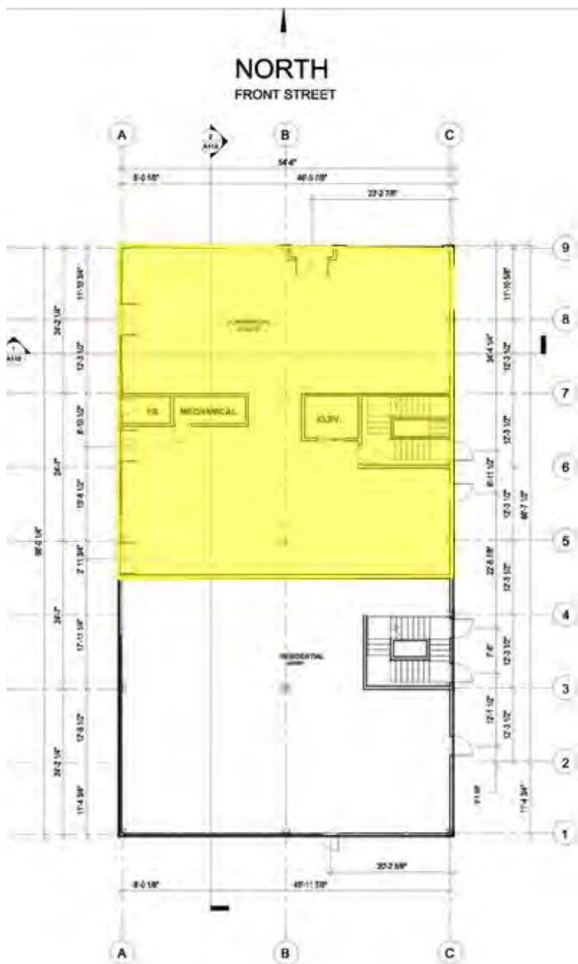
1 GROUND FLOOR PLAN 1/8" = 1'-0"
