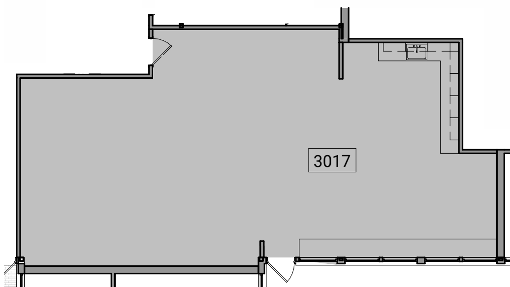
2 Suite 3017 - Partial Existing Level 1 Floor Plan 3017 8' 16' 24' 3/32" = 1'-0"
