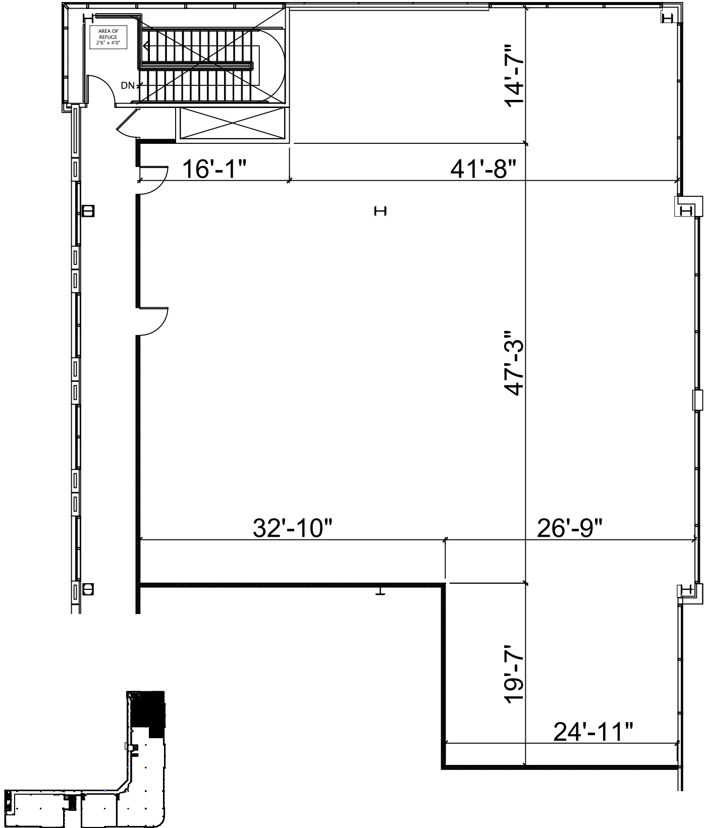
2ND FLOOR KEY PLAN
