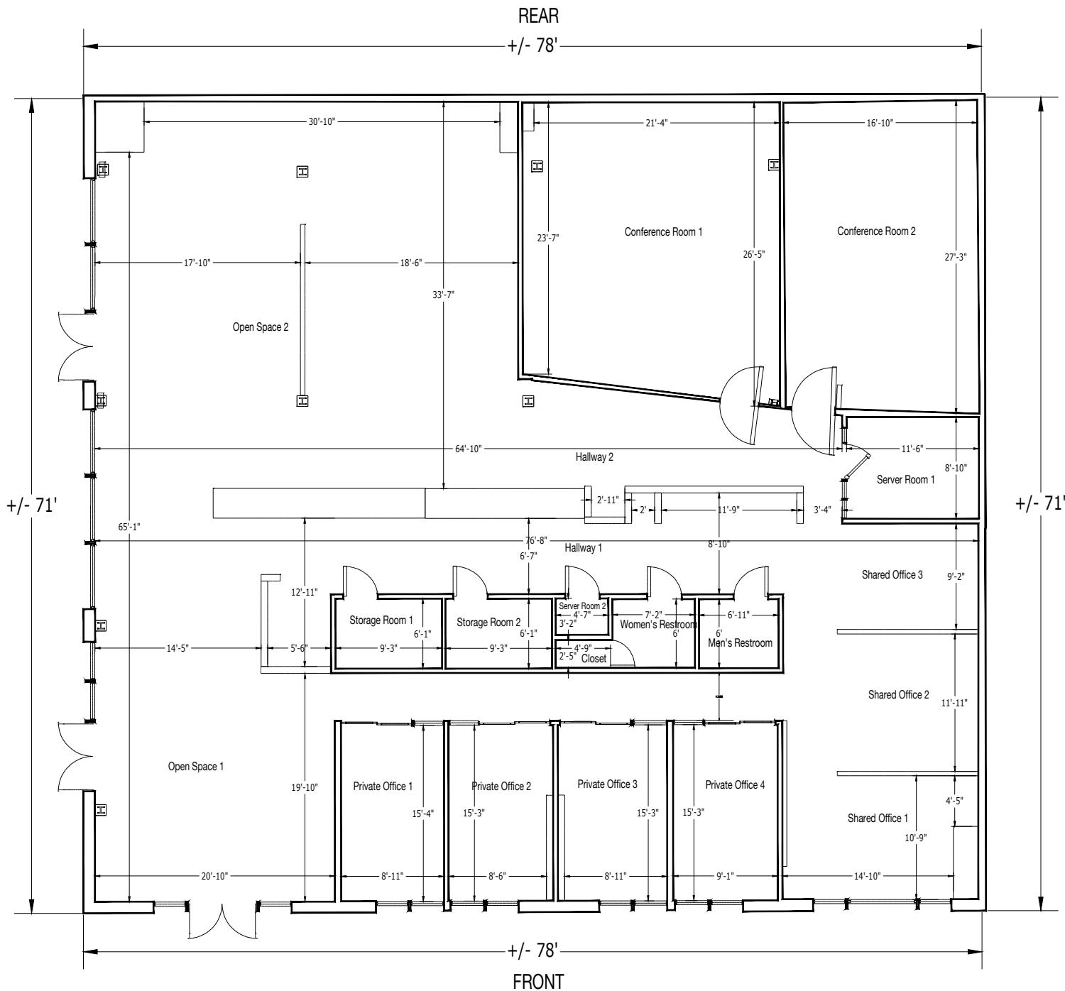
1 MAIN FLOOR
