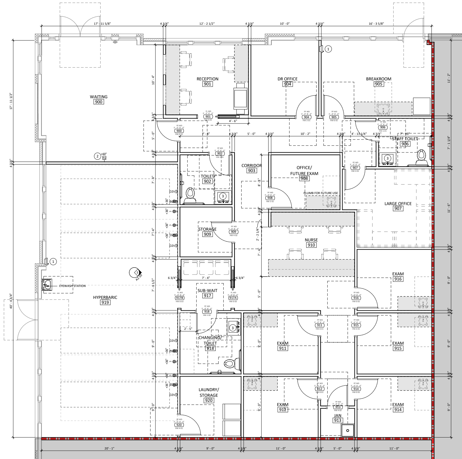
1 FLOOR PLAN - FLOOR 1
