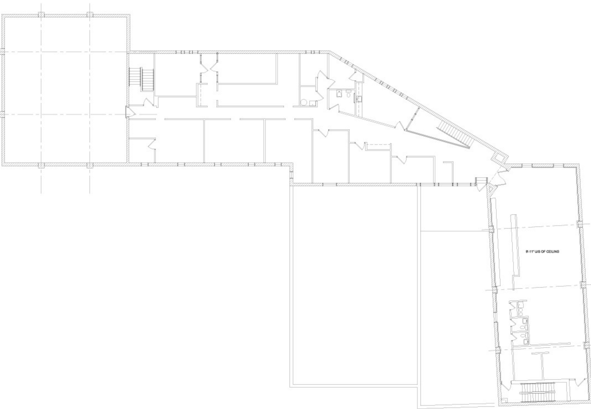
1 Existing Conditions @ SECOND FLOOR A2.02 SCALE: 3/8" = 1'-0"
