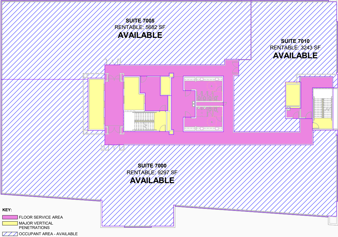
① LEVEL 7 1/16" = 1'-0"
