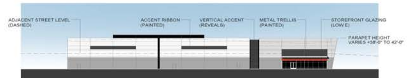
South Elevation
