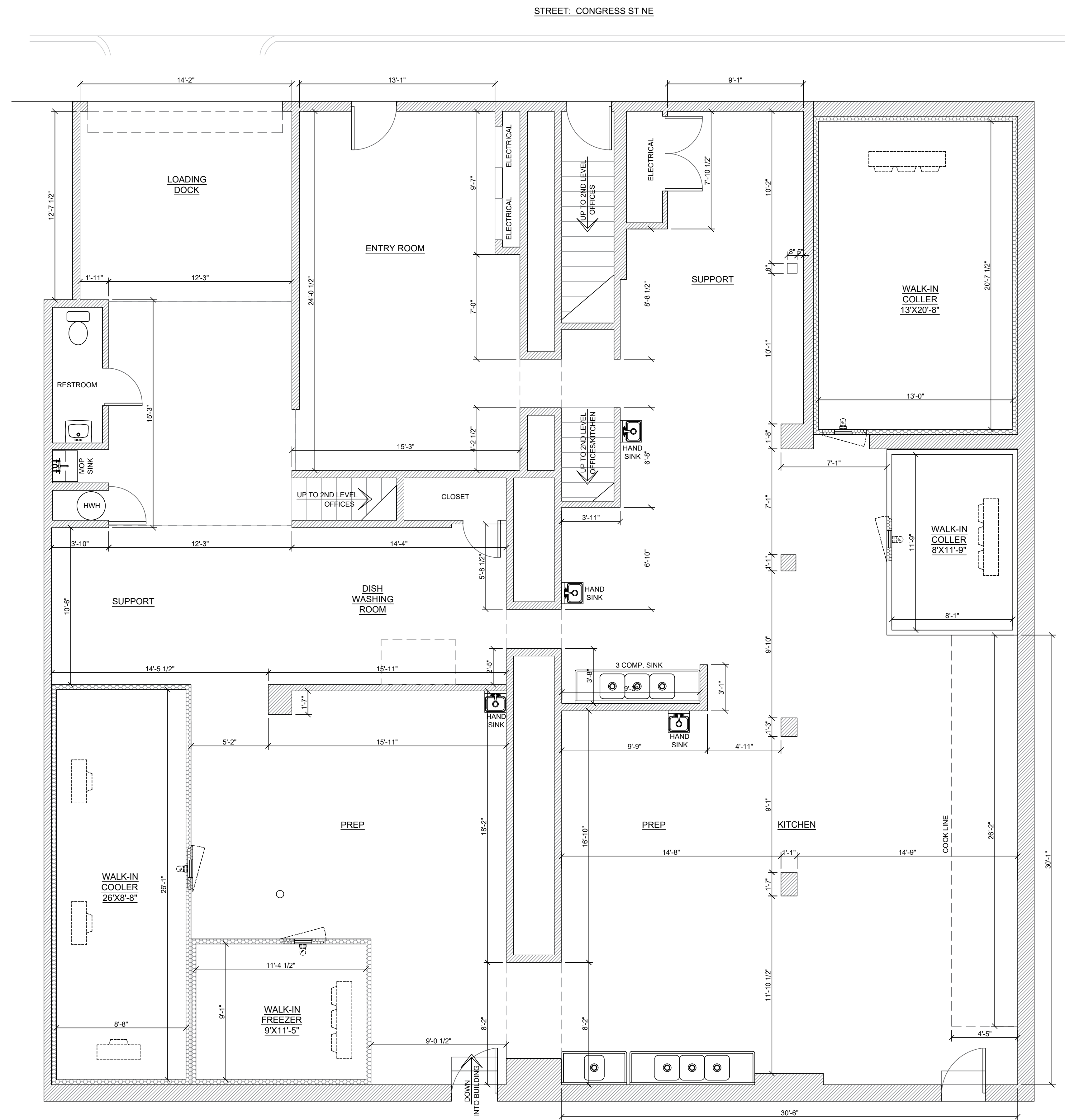
1 FIRST FLOOR BUILDING LAYOUT SCALE: 1/4" = 1'-0"
