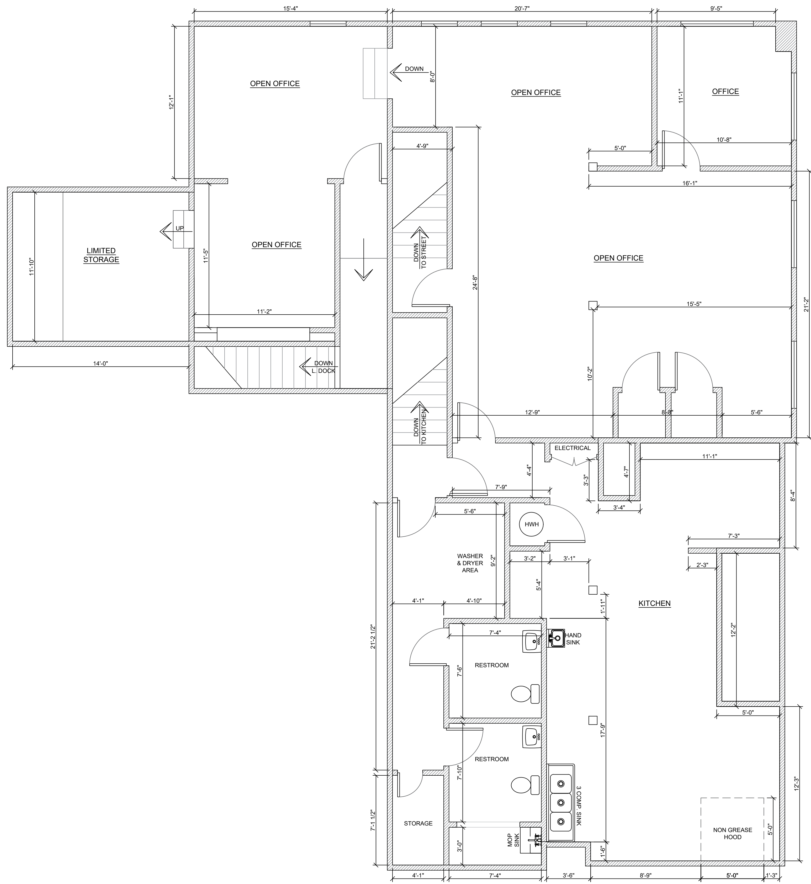
2 SECOND FLOOR BUILDING LAYOUT SCALE: 1/4" = 1'-0"
