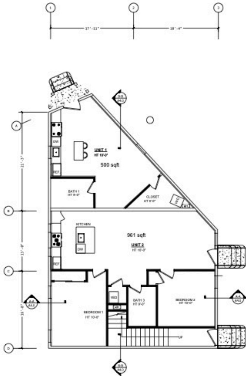
1 PROPOSED 1ST FLOOR PLAN
