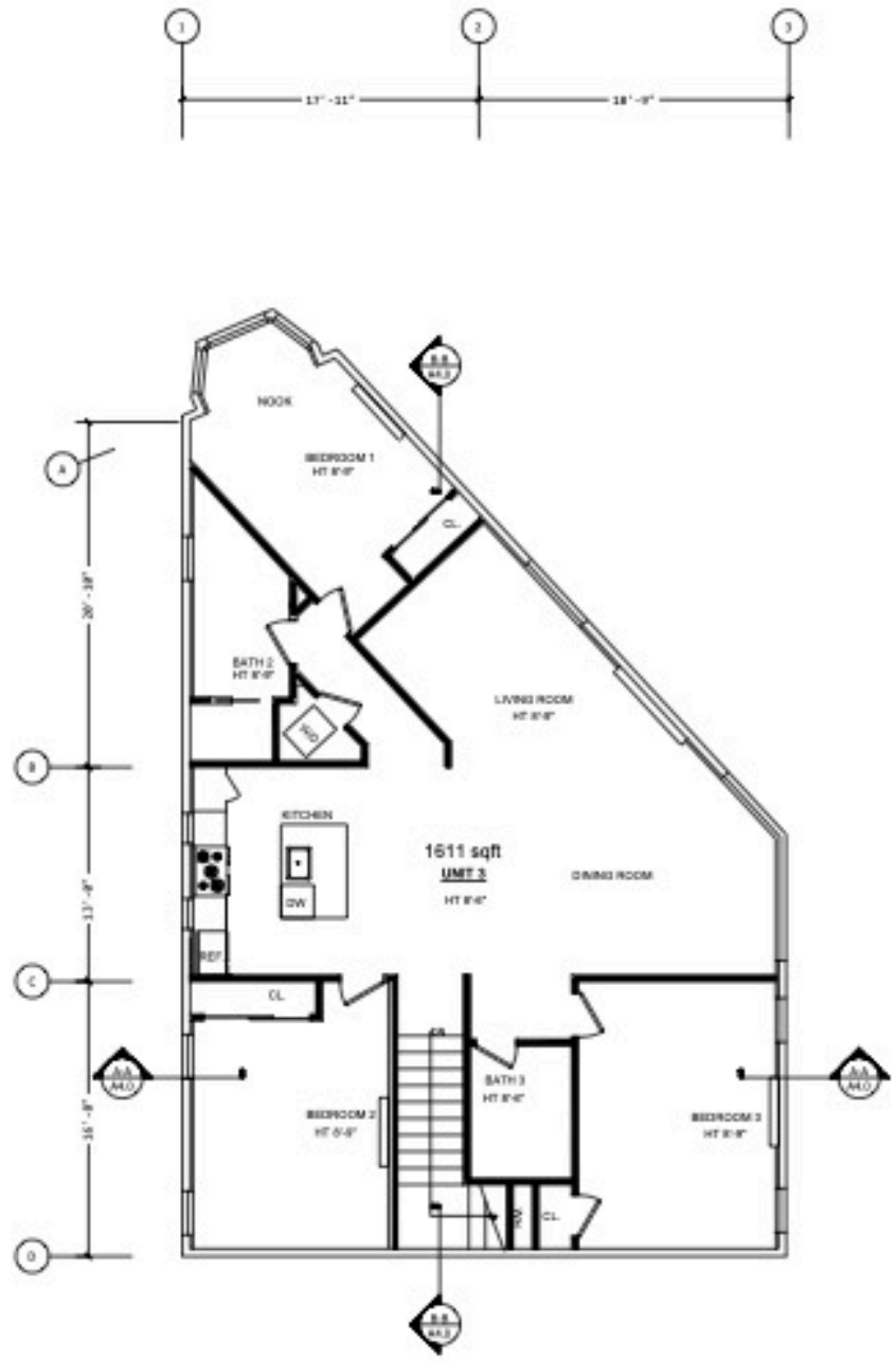
2 PROPOSED 2ND FLOOR PLAN
