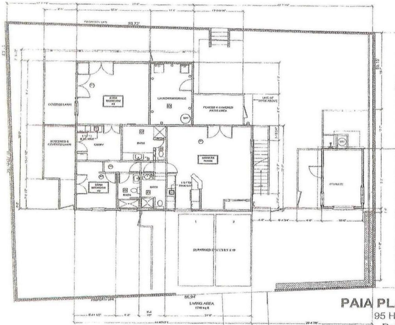
1 FIRST FLOOR PLAN - STRH LAYOUT NTS
