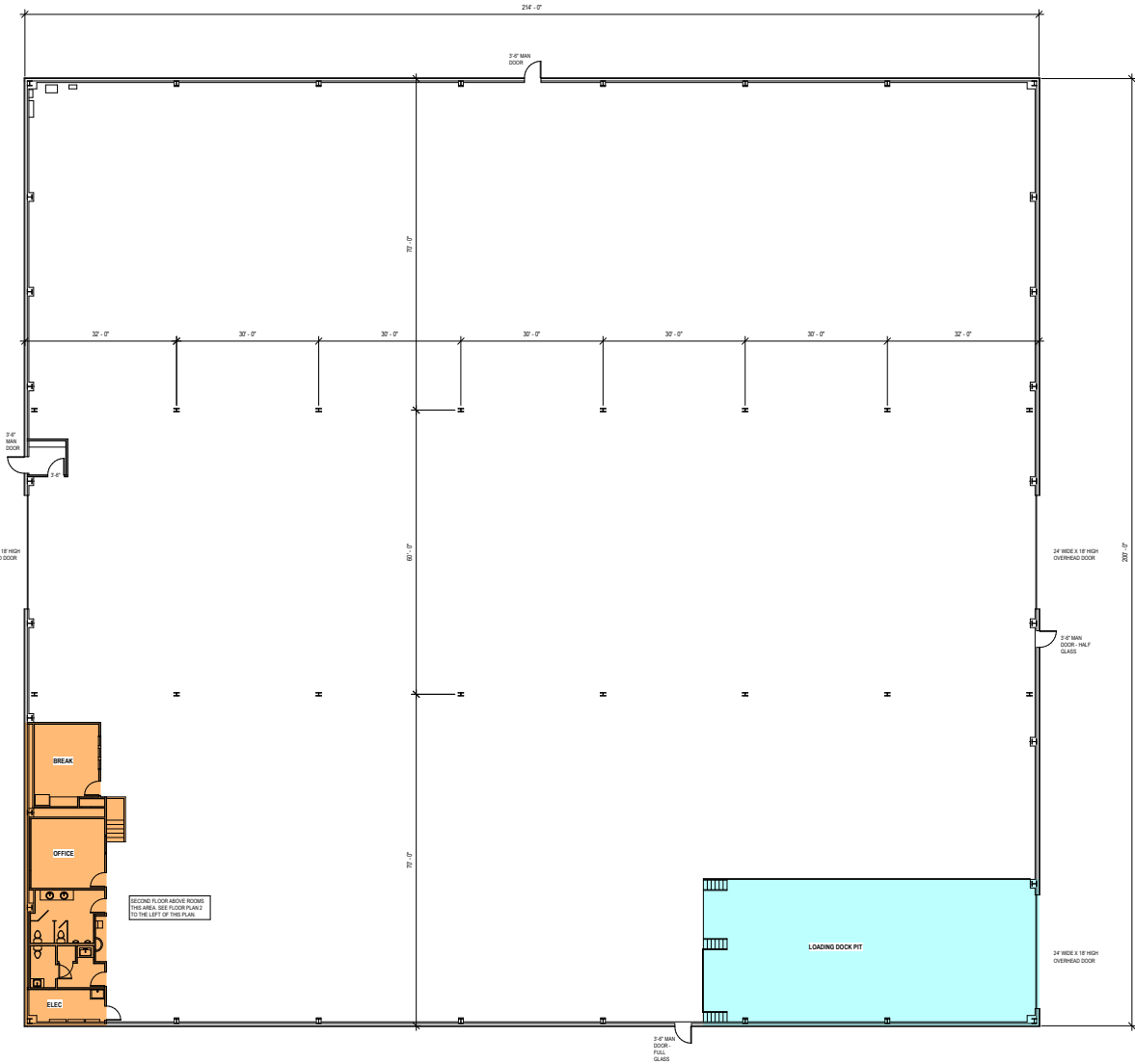
1 FLOOR PLAN SCALE: 3/32" = 1'-0"
