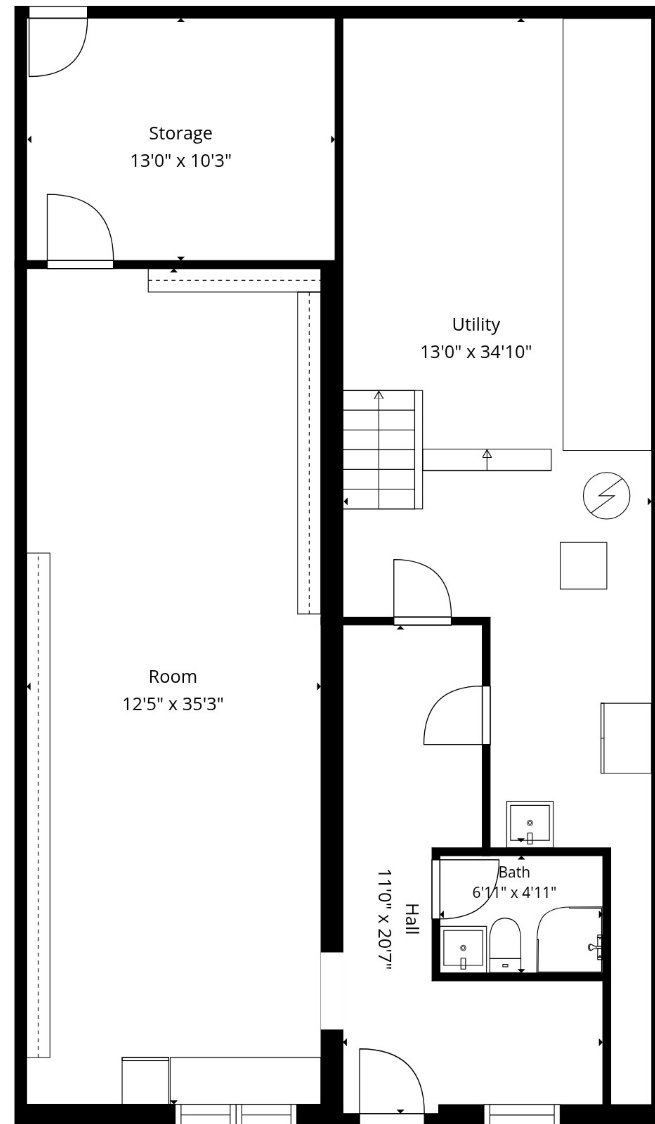
Basement
