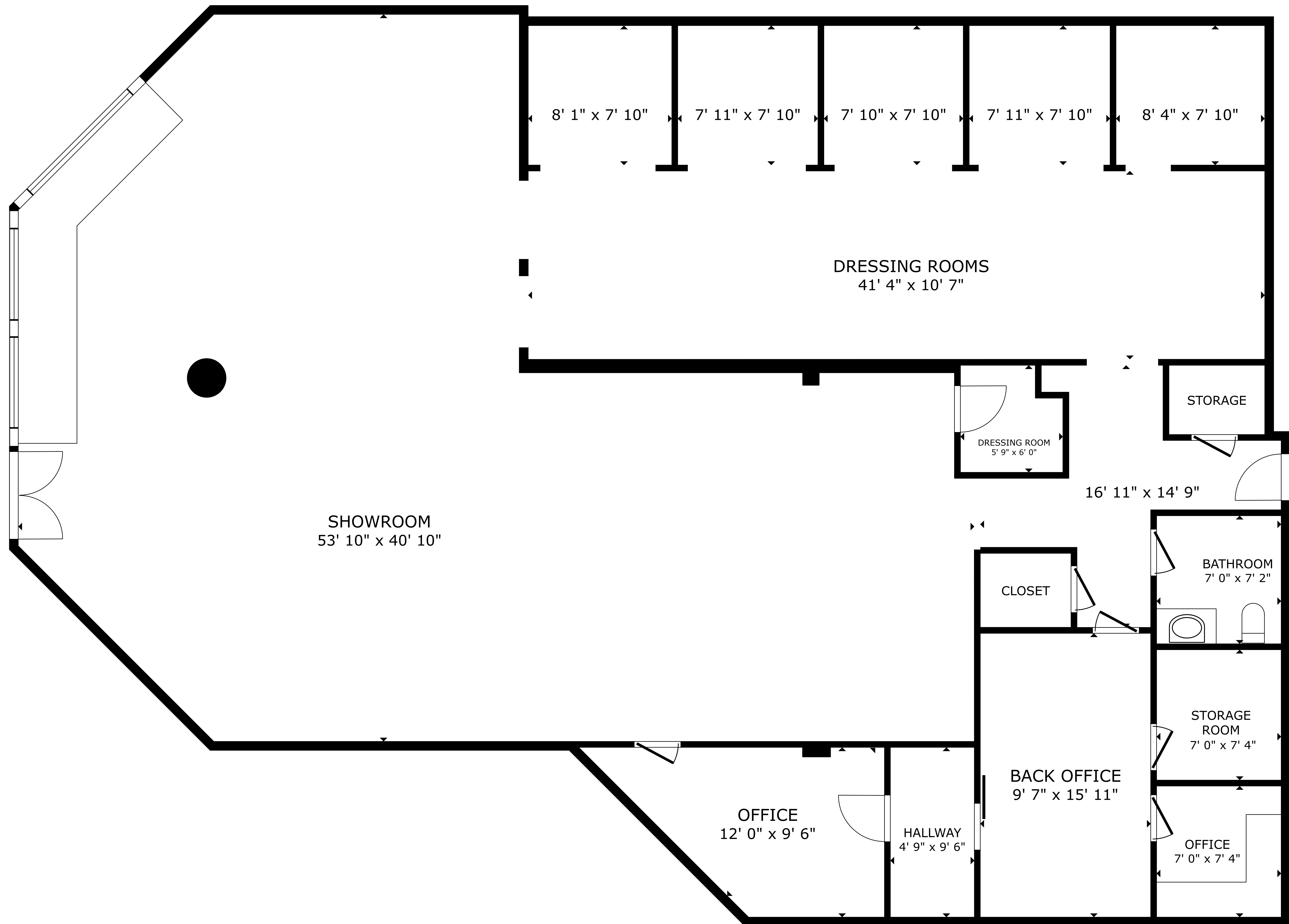
FLOOR PLAN
