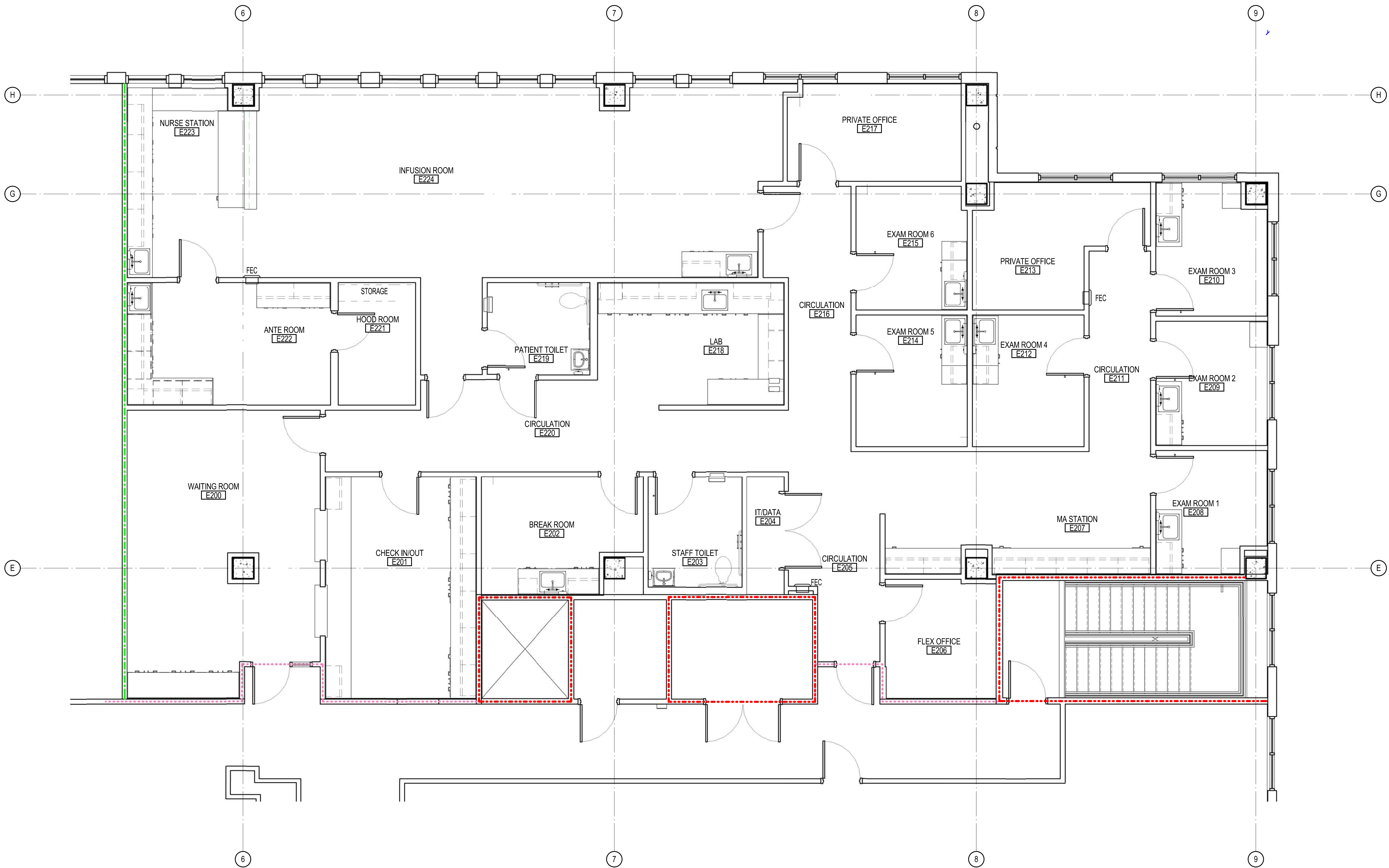
01 FLOOR PLAN - STE. 470 1/4" = 1'-0"
