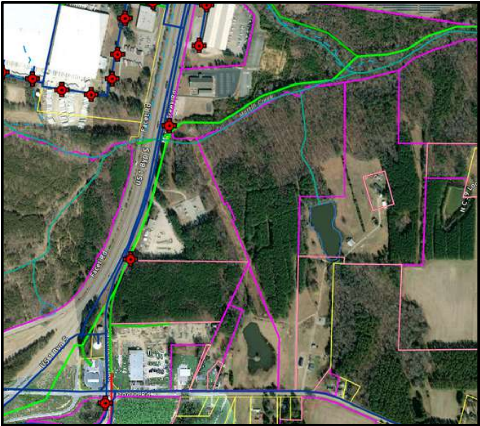
UTILITIES MAP
