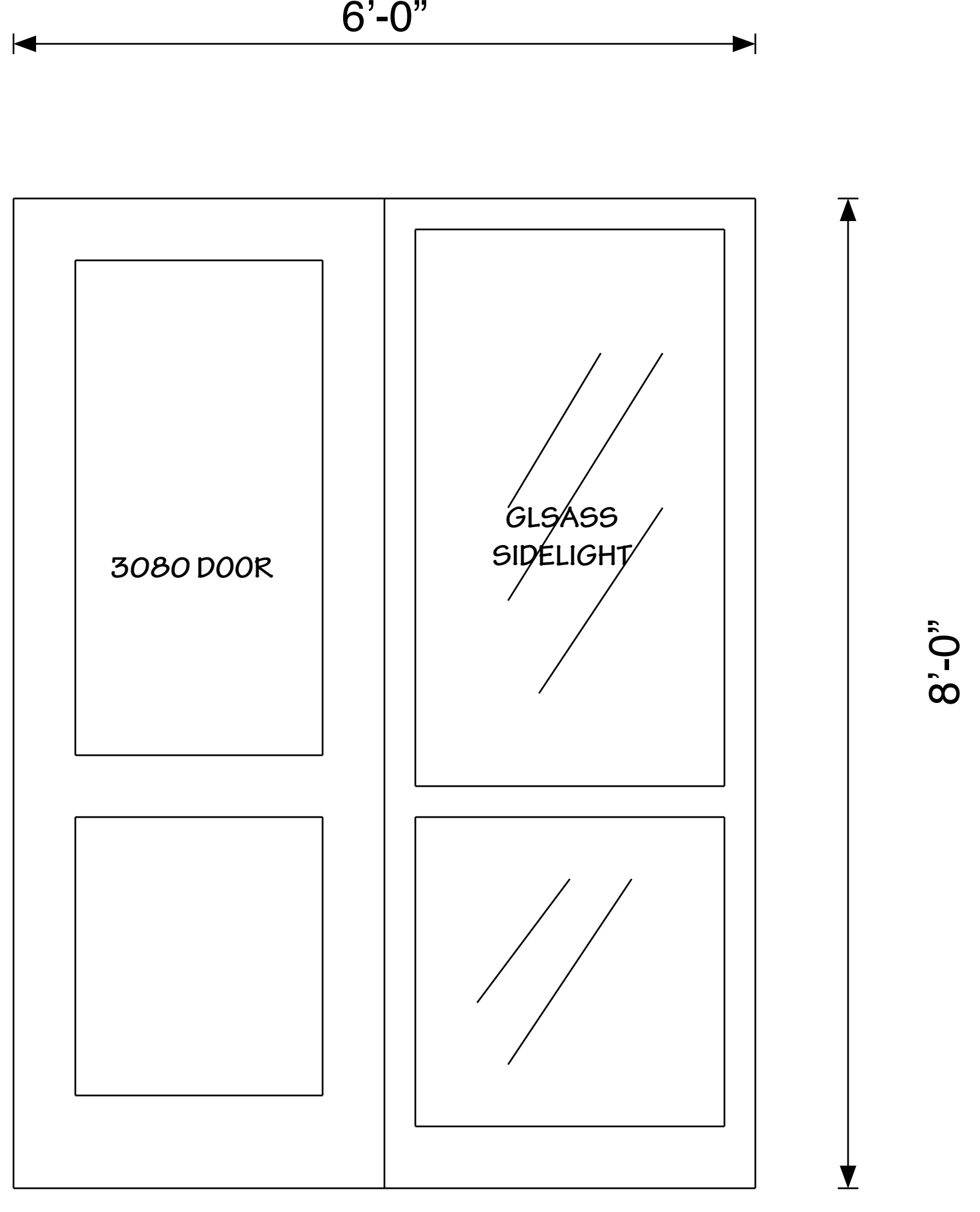
OFFICE DOOR ELEVATION
