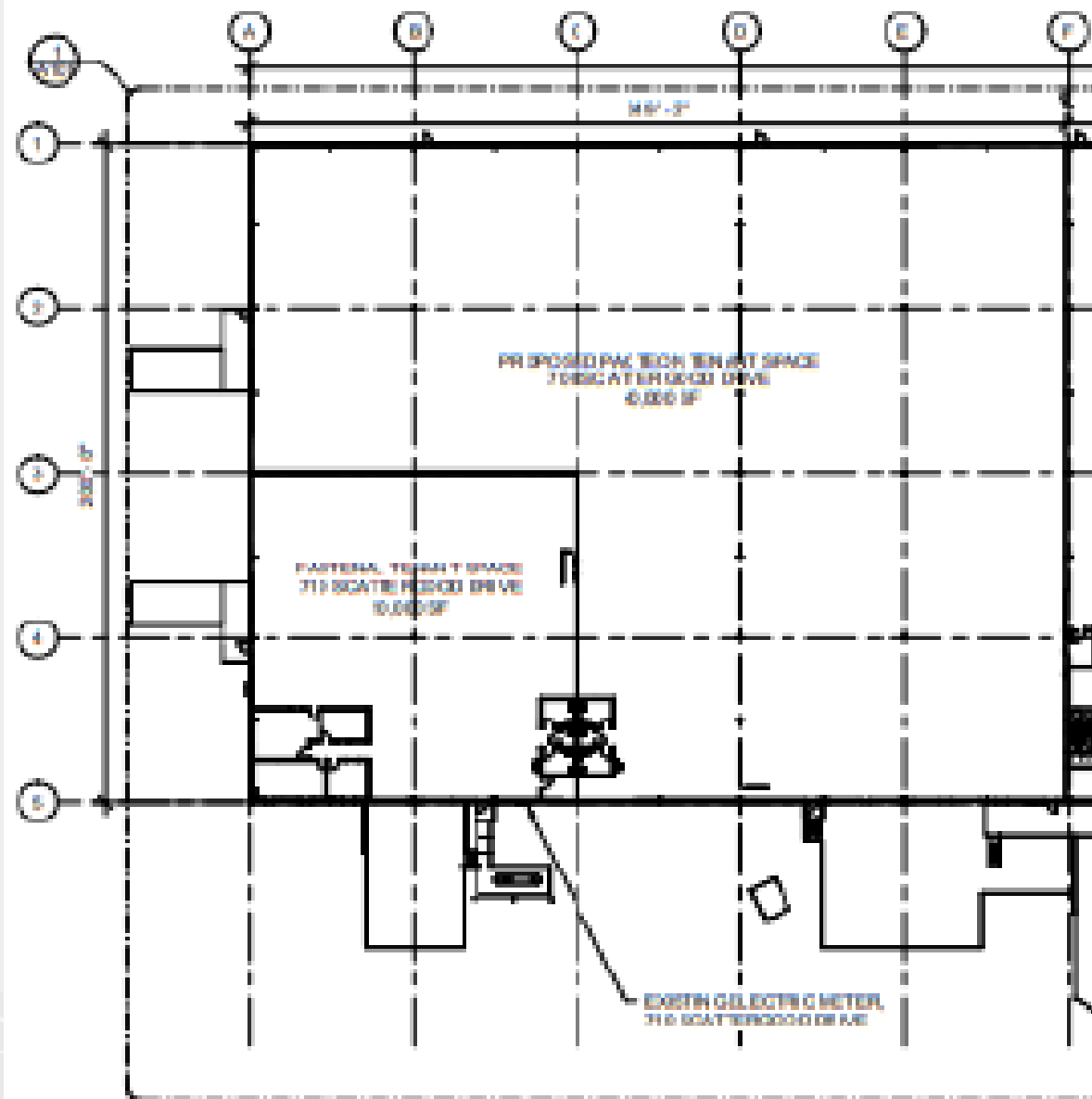
1 FLOOR PLAN - OVERALL BUILDING A 100 1" = 30'-0"
