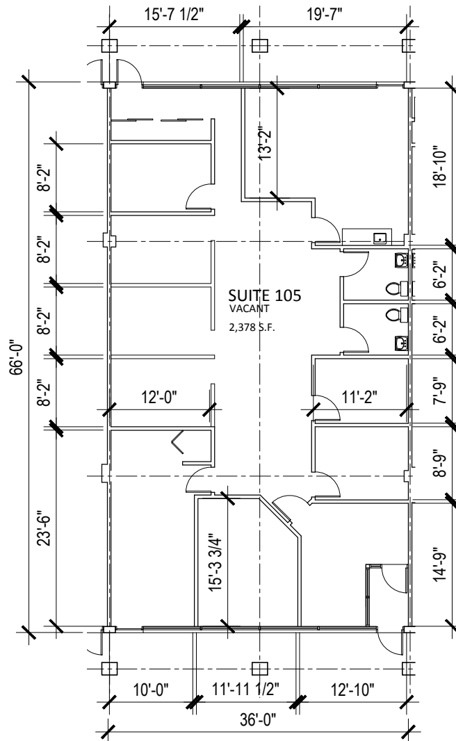
FLOOR PLAN 1/16"=1'-0" N
