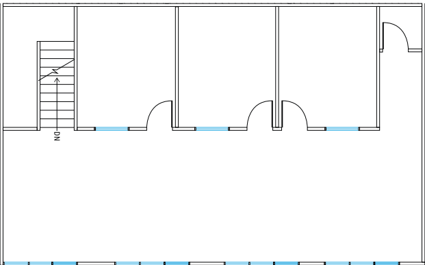
EXISTING SECOND STORY FLOOR PLAN
