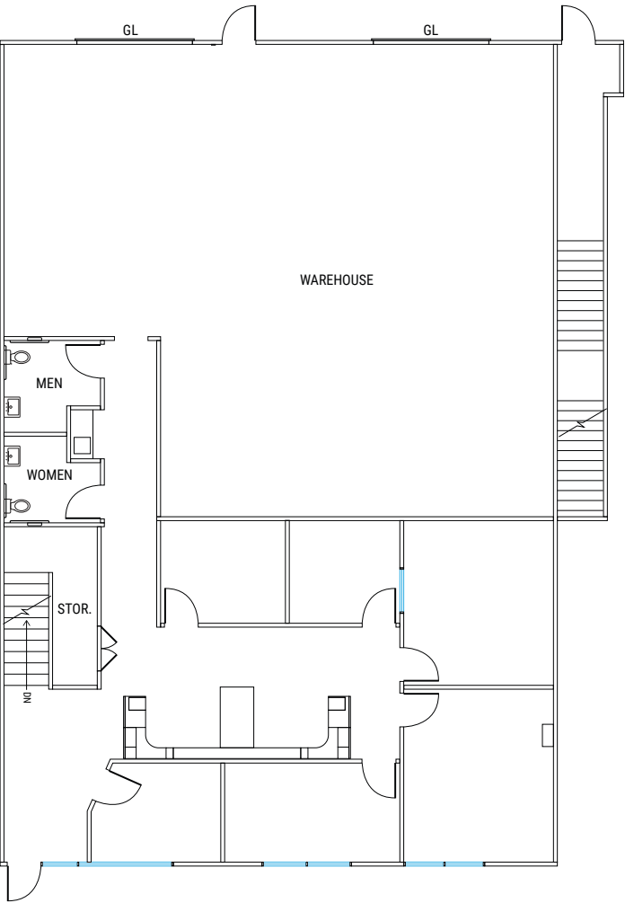
EXISTING SECOND STORY FLOOR PLAN
